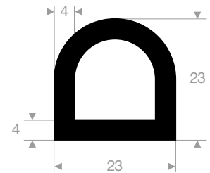
VR21500423 TPE 60° Shore black roll length 25 meter Price: 12,00 €/m+VAT
