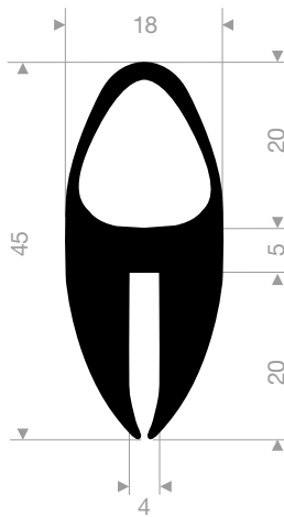
VR21109004 EPDM 65° Shore black roll length 50 meter Price: 12,00 €/m+VAT
